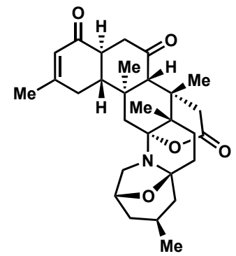
Norzoanthamine
