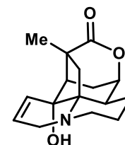
Annotinolide D
