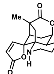
Annotinolide C
