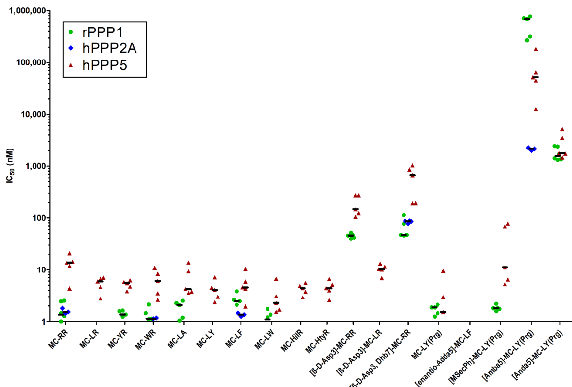
Fig. S6: Comparison of IC_{50} values on the three tested phosphatases Biological replicates were plotted individually using GraphPad Prism 5 and individual IC_{50} are noted. Black bars show the median of the IC_{50} .
